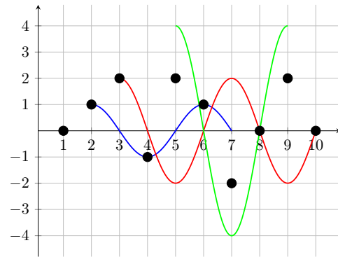
Figure I.1: Interference of three waves in Sample Input 2. The black dots represent the resulting wave's height.
