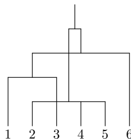
Figure 3: A messy dendrogram
