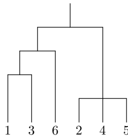
Figure 2: An example dendrogram
